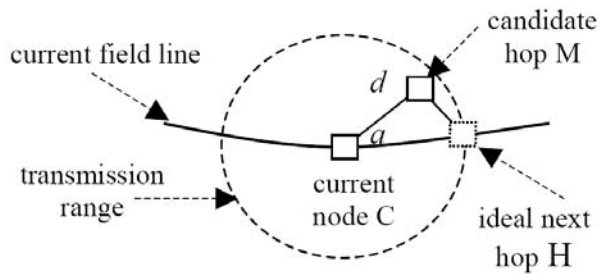
Figure 2: Finding the Ideal Next Hop
