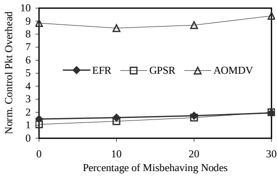
Figure 6(d): Normalized Control Overheads
