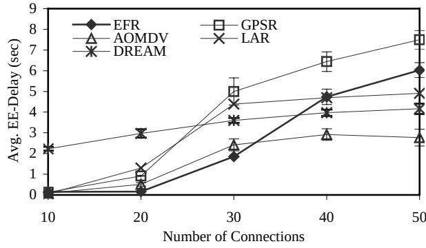
Figure 4(b): Average End-to-End Delay
