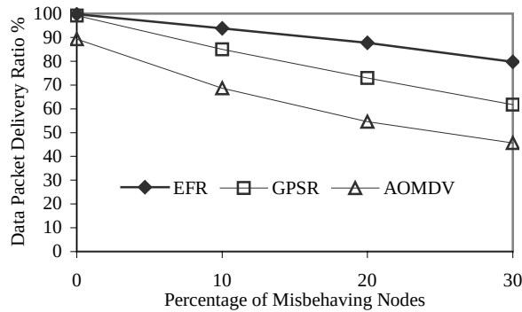
Figure 6(a): Data Packet Delivery Ratio
