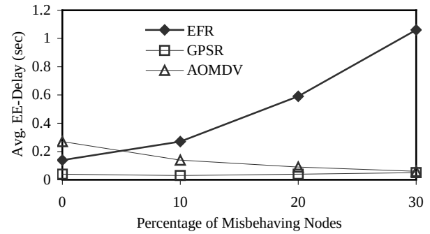
Figure 6(b): Average End-to-End Delay
