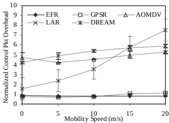
Figure 3(c): Normalized Control Overhead
