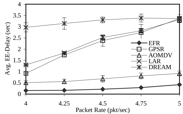
Figure 5(b): Average End-to-End Delay
