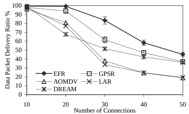
Figure 4(a): Data Packet Delivery Ratio
