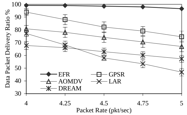
Figure 5(a): Data Packet Delivery Ratio
