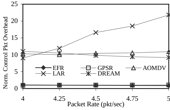
Figure 5(c): Normalized Control Overhead
