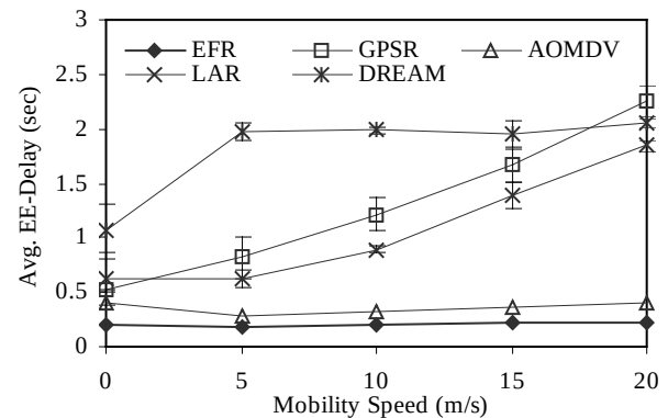
Figure 3(b): Average End-to-End Delay
