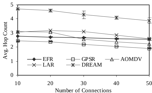
Figure 4(d): Average Hop Count
