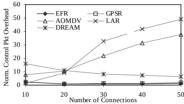
Figure 4(c): Normalized Control Overhead
