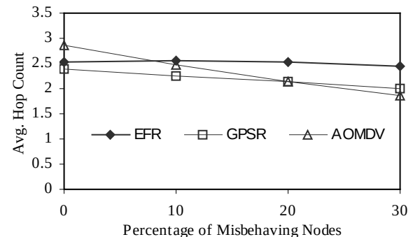
Figure 6(c): Average Hop Count
