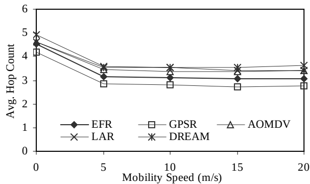
Figure 3(d): Average Hop Count
