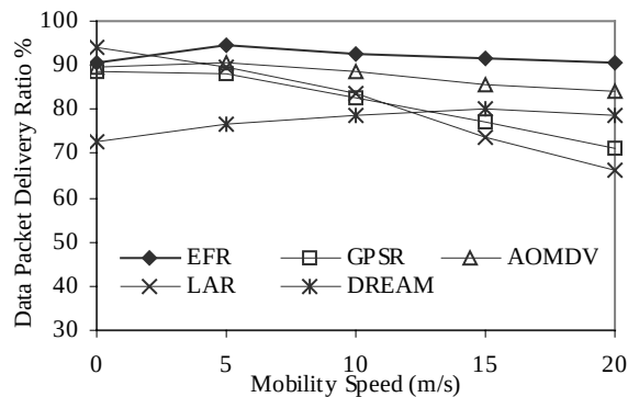
Figure 3(a): Data Packet Delivery Ratio (confidence intervals omitted for readability)
