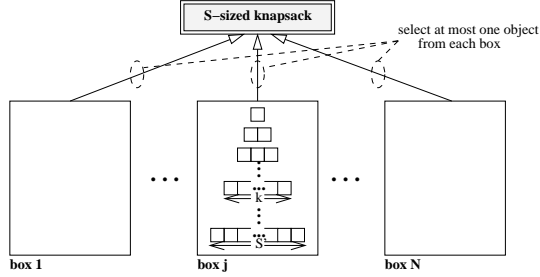
Figure 1: The packing problem involved in the composition step.
