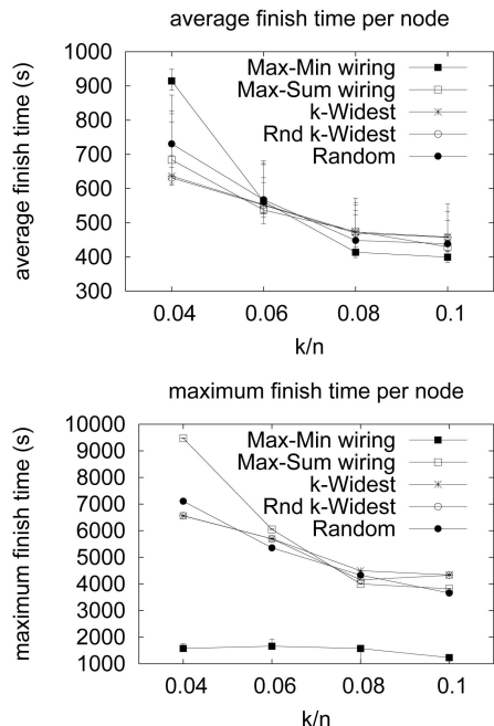
Fig. 11. Simulation of a closed overlay network based on Sprint physical topology in the presence of a very slow node.
