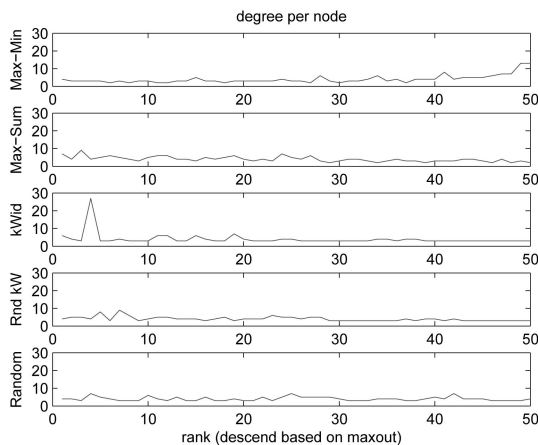
Fig. 9. Node degree on different overlay topologies for k/n = 0.04 .
