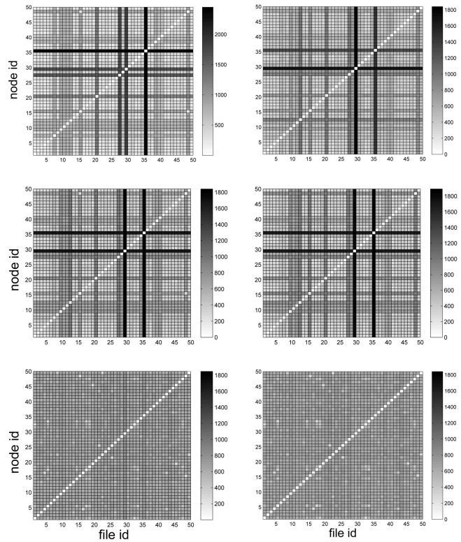
Fig. 13. Maximum finish time for all nodes and all files under different wirings (from left to right): MaxSum, Random, k-Widest, Rnd k-Widest, MaxMin strategies with cooperative nodes, and Max-Min with upload-selfish slowest node ( k/n = 0.04 ).
