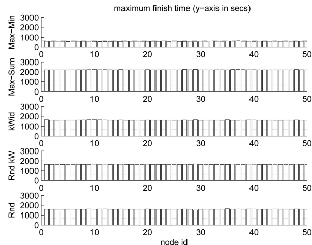
Fig. 7. Maximum finish time per node based on Sprint physical topology with link density k/n = 0.04 . The horizontal dashed line indicates the maximum finish time on the Max-Min topology.
