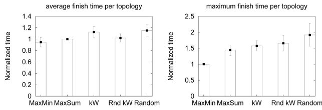
Fig. 3. PlanetLab experiment and performance evaluation of different wiring strategies.
