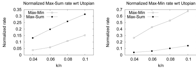
Fig. 8. Normalized Max-Sum and Max-Min rate with respect to the Utopian one based on Sprint physical topology.
