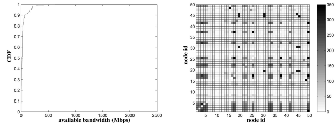
Fig. 4. Sprint physical topology, empirical CDF, and scatter plots of available bandwidths.
