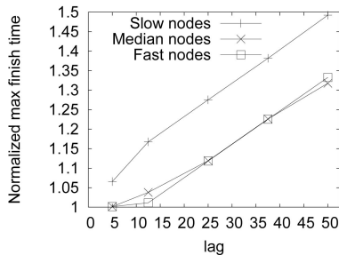
Fig. 15. Normalized maximum finish time when a set of nodes is delayed in Max-Min topology with respect to the maximum finish time when all the file requests are synchronized and the file is immediately available. The lag is a percentage of the maximum finish time of the reference setting.
