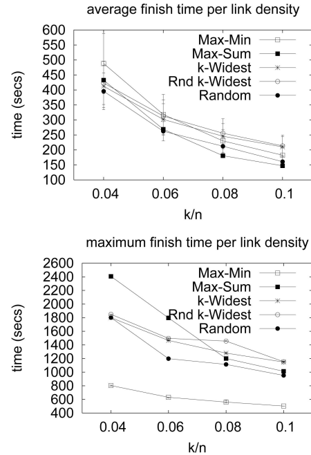
Fig. 6. Simulation of a closed overlay network based on Sprint physical topology.
