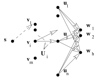
Fig. 17. Reduction from MAX-UNIQUES( k ) to Max-Sum.
