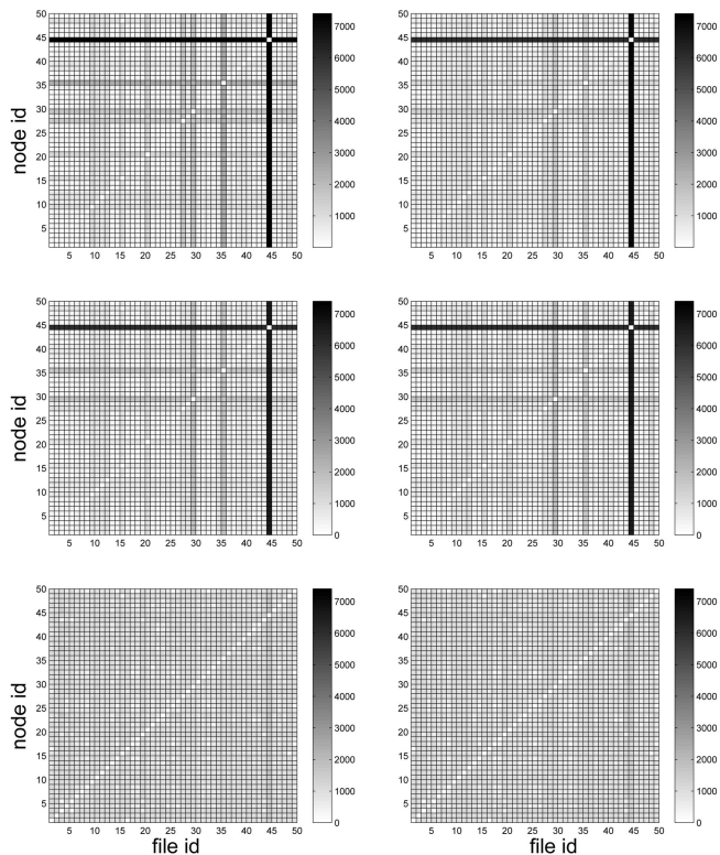
Fig. 14. Maximum finish time for all nodes and all files under different wirings (from left to right): MaxSum, Random, k-Widest, Rnd k-Widest, MaxMin strategies with cooperative nodes, and Max-Min with upload-selfish slowest node, in the presence of a very slow node ( k/n = 0.04 ).
