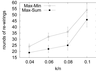
Fig. 5. Sprint physical topology and speed of convergence to a stable overlay topology with 50 overlay nodes using different peer-selection policies.
