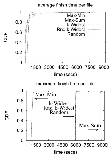
Fig. 12. CDF for the average and maximum finish time per file per node for link density k/n = 0.04 , in the presence of a very slow node.
