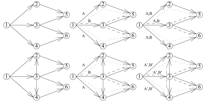
Fig. 1. Mixing max-flows. Left: empty network. Middle: RF(1, 5) and RF(1, 6) coexisting. Right: RF(1, 2), RF(1, 3), RF(1, 4), RF(1, 5), RF(1, 6) coexisting. Top: initial network. Bottom: Initial augmented with edges, (3,2) and (3,4).
