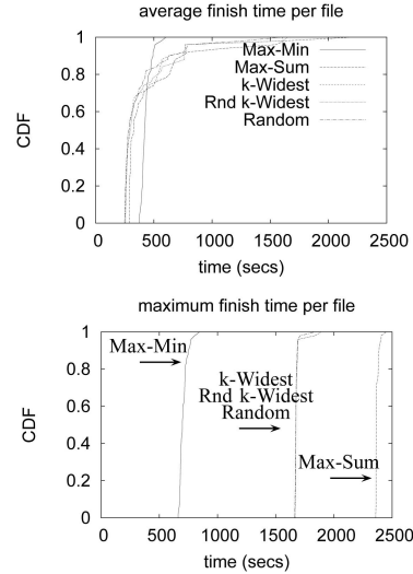
Fig. 10. CDF for the average and maximum finish time per file per node for link density k/n = 0.04 .
