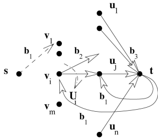
Fig. 16. Reduction from MAX-UNIQUES( k ) to Max-Min.
