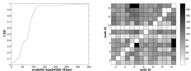
Fig. 2. PlanetLab experiment, empirical CDF, and scatter plots of available bandwidths.
