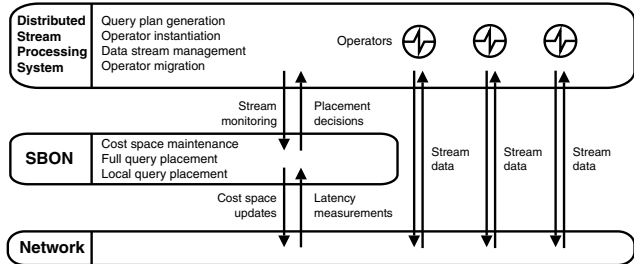
Figure 2. Architecture Overview
