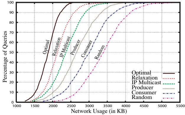
Figure 8. Network usage
