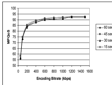
Figure 4. The MPQoS vs. Bit rate curves for real video clips with talk show content.
