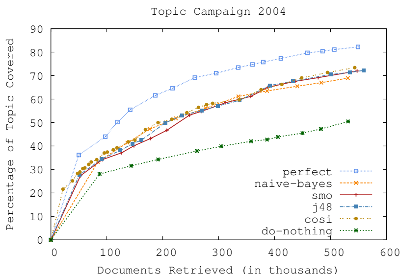
Fig. 7: Results of the six policies for topic Campaign-2004 of NYT Corpus
