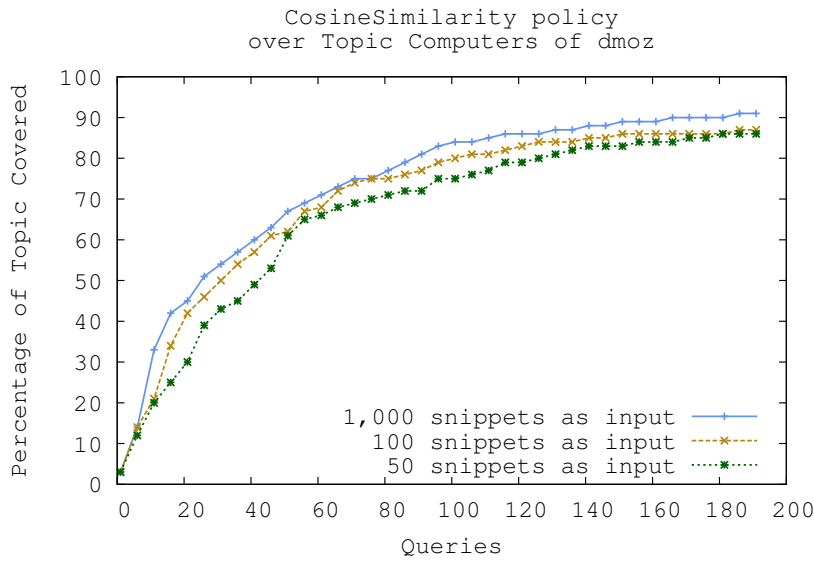
Fig. 15: Impact of the input document size using CosineSimilarity on topic Computers
