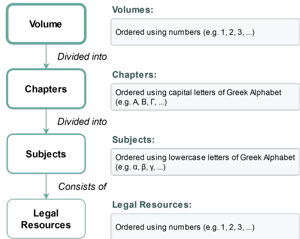
Figure 1: Original GLC thematic hierarchy
