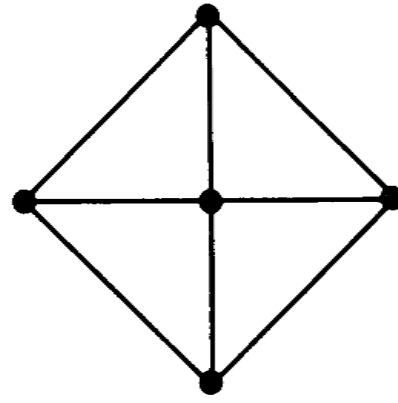
Fig. 7. A graph that is not 3-regular.
