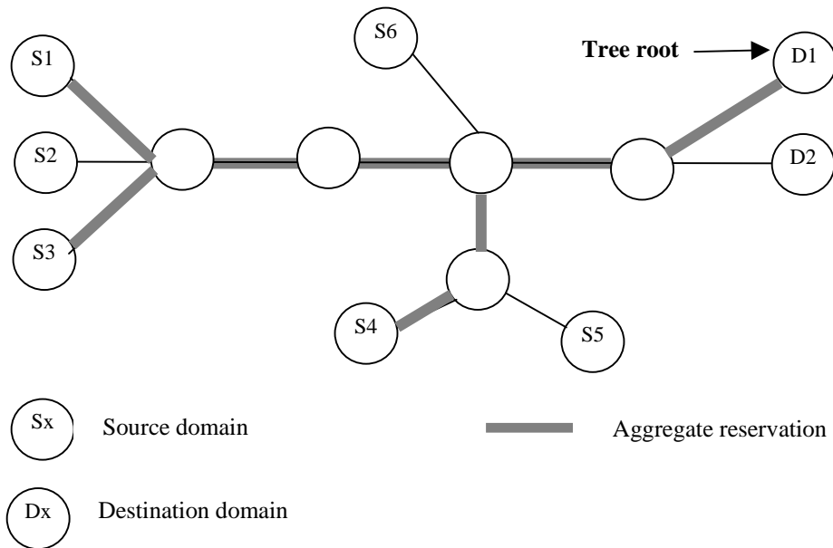
Figure 10. BGRP example: individual reservations from S1, S3 and S4 towards destination D1 are aggregated into an aggregate reservation tree with root D1
