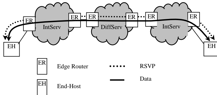
Figure 9. End-to-end inter-domain RSVP usage
