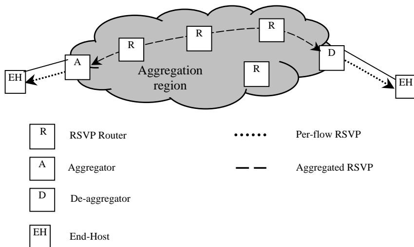
Figure 7. RSVP aggregation
