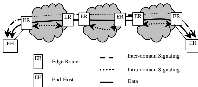
Figure 5. Two-tier QoS Signaling
