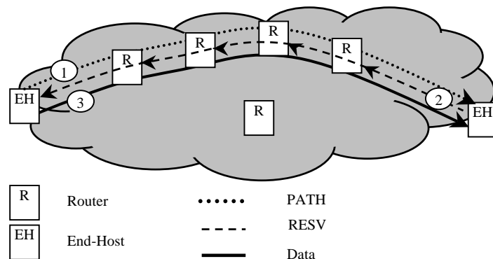
Figure 2. RSVP message exchange
