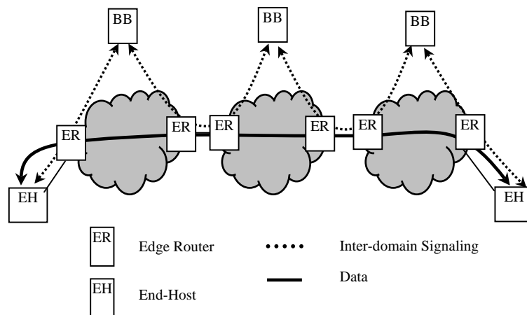
Figure 13. Inter-domain QoS signaling in BB architectures
