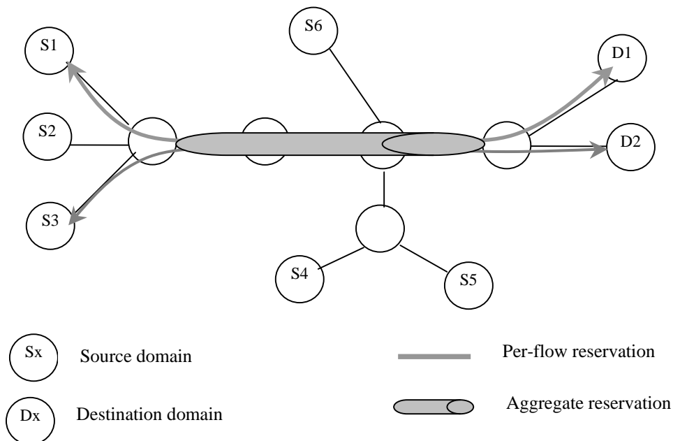
Figure 12. DARIS example: individual reservations from S1 and S3 towards destinations D1 and D2 respectively are aggregated into an aggregate reservation along their common path segment
