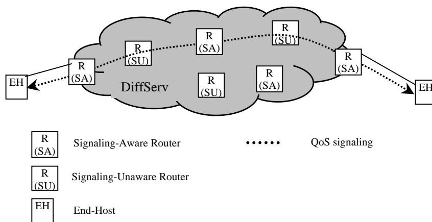
Figure 6. Dynamic Resource Management inside a DiffServ domain
