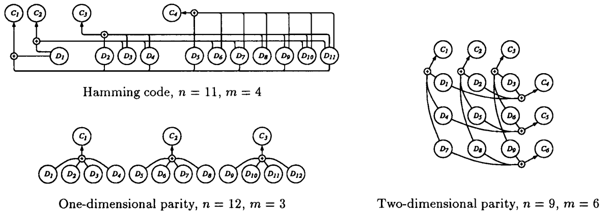
Figure 8. Parity-based encodings
