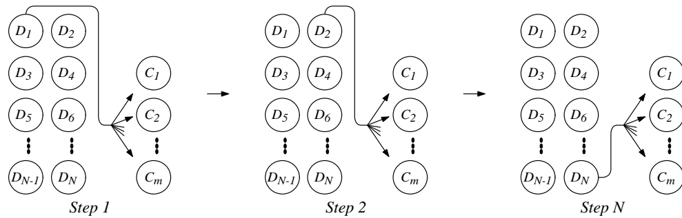
Figure 6. The broadcast algorithm
