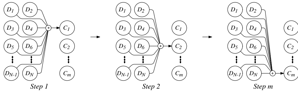
Figure 7. The Fan-in algorithm
