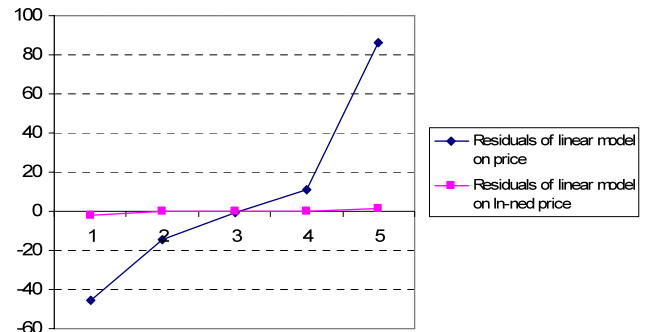
Fig. 4 Residuals
