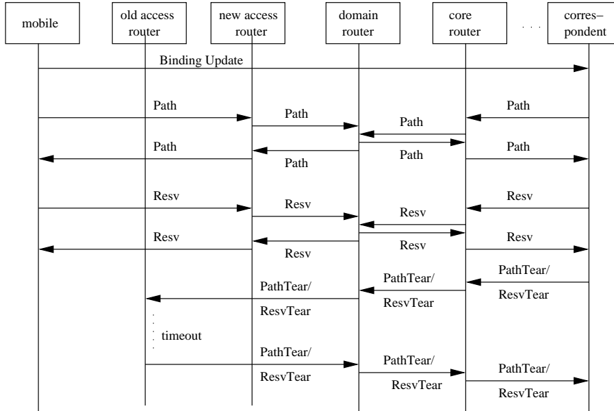
Figure 2: Analytical RSVP signaling after a handoff
