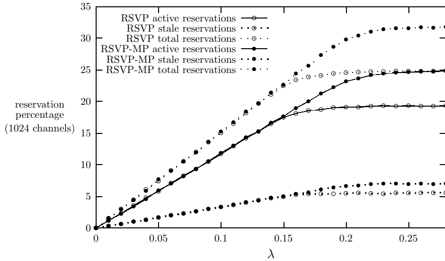
Figure 10: Active and stale reservations in the internal interfaces of the edge router vs new arrivals \lambda ( v = 1m/sec )
