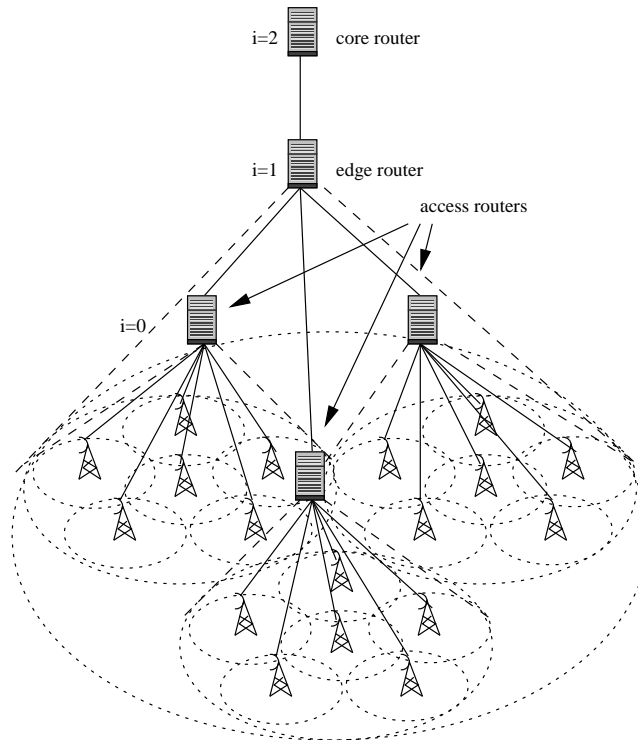
Figure 6: Access Network Topology
