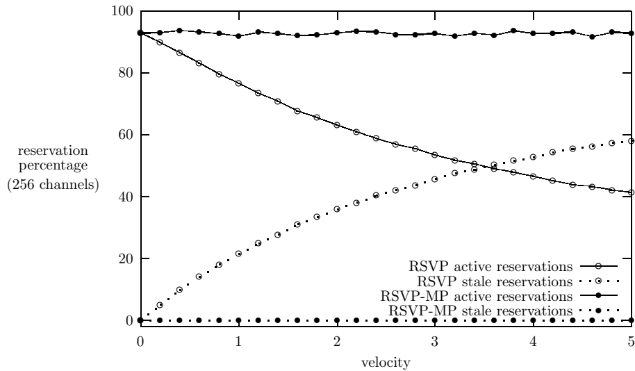
Figure 11: Active and stale reservations in the link between the edge and the core router vs velocity ( \lambda = 0.2 )
