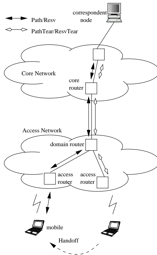
Figure 1: Network topology
