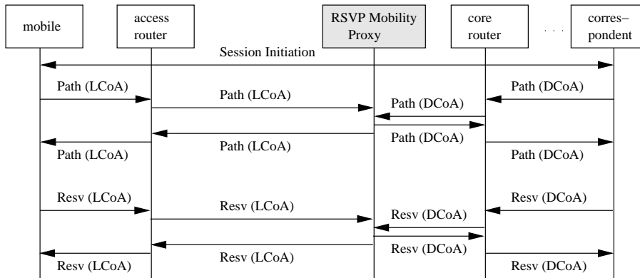
Figure 4: RSVP signaling through the RSVP Mobility Proxy
