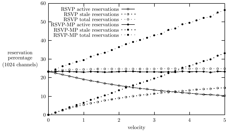
Figure 12: Active and stale reservations in the internal interfaces of the edge router vs velocity ( \lambda = 0.2 )
