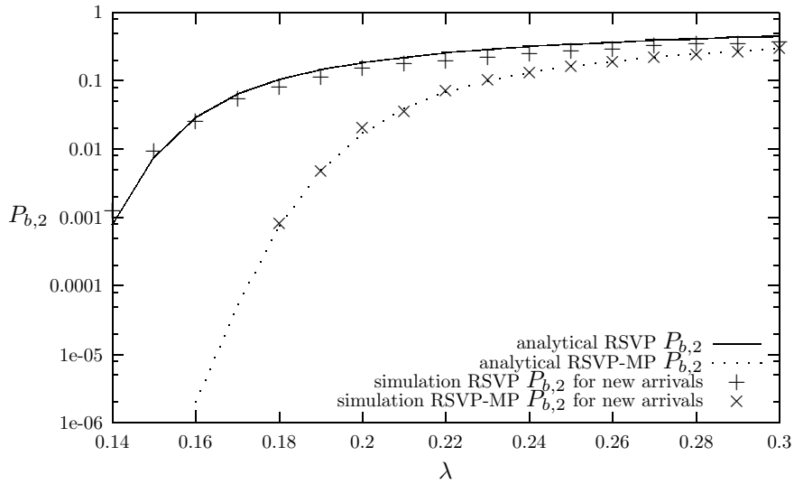
Figure 7: Blocking Probability vs new arrival rate \lambda ( v = 1\text{m/sec} )
