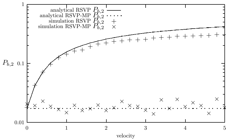
Figure 8: Blocking Probability vs velocity ( \lambda = 0.2 )
