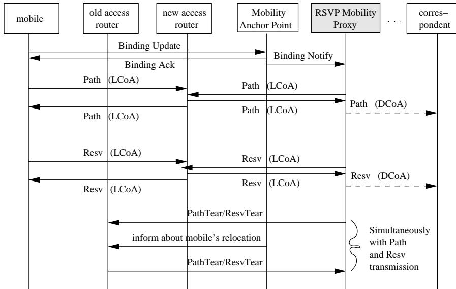
Figure 5: RSVP reservation signaling through the RSVP-MP after a handoff
