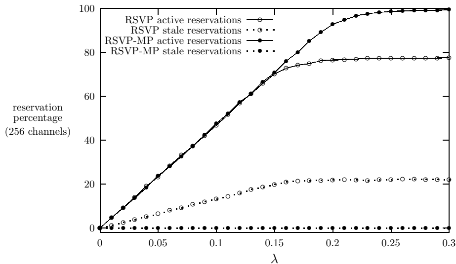
Figure 9: Active and stale reservations in the link between the edge and the core router vs new arrivals \lambda ( v = 1m/sec )
