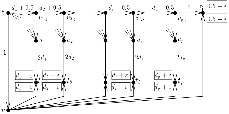
Fig. 8. A bad instance for the maximum routable demand. Only part j of the graph is represented. Demand values are indicated within rectangle boxes.
