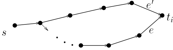
Fig. 4. End of constructing a backward path.
