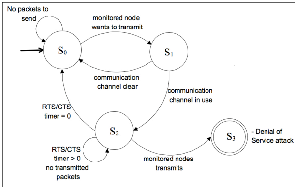
Fig. 4. 802.11 MAC protocol specifications.
