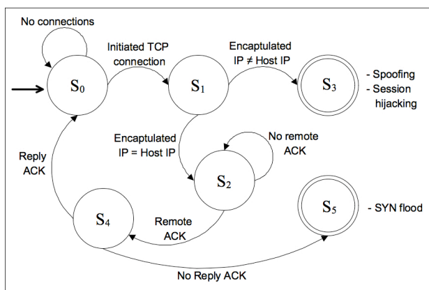
Fig. 2. Transport layer specifications.
