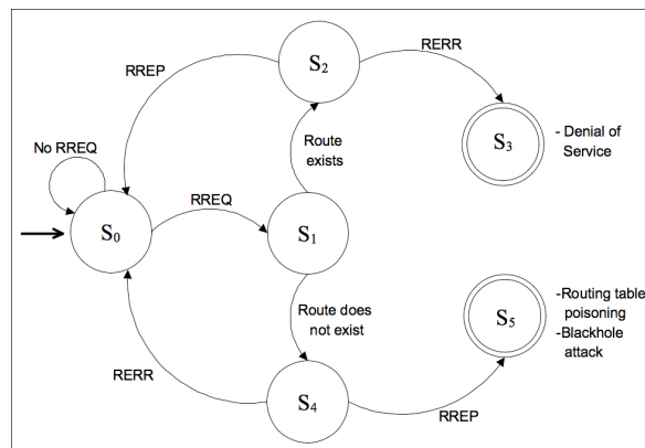
Fig. 3. AODV monitoring specifications.
